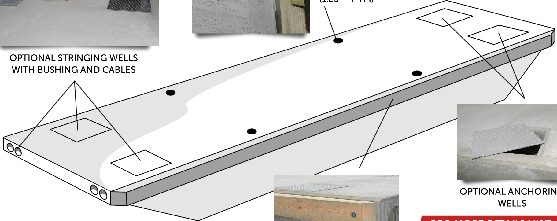
STANDARD LIFTING SOCKETS (1.25" - 7 TPI)
